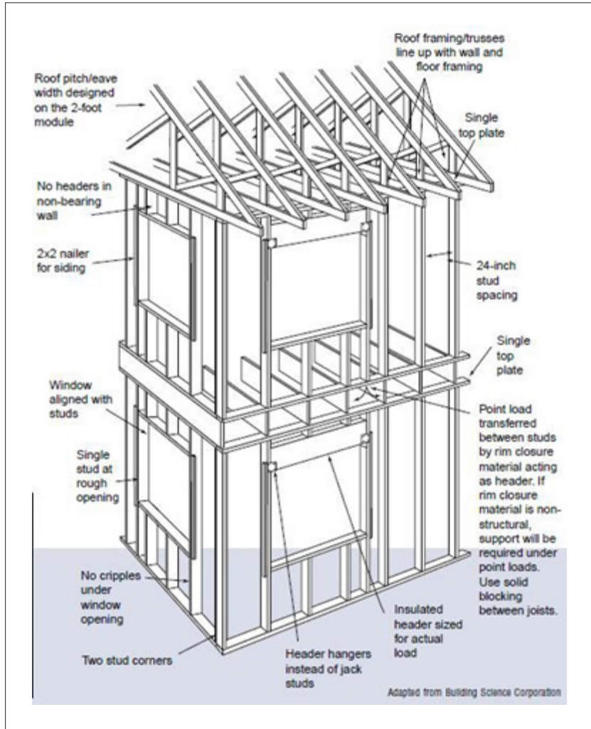
Advanced Framing
